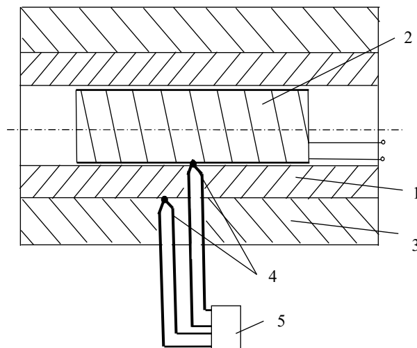
Fig. 2. Device for researching the thermal conductivity of wood polymer material: 1 – wood polymer material; 2 – cylindrical heater; 3 – thermal insulation; 4 – thermocouples; 5 – temperature recording device
