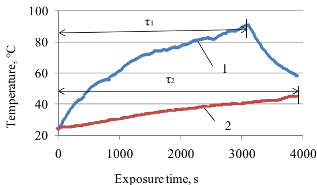
Fig. 6. Results of determining the temperature on the surface of a wood polymer material when heated to 90 °C: 1 – heating curve; 2 – temperature value on the inverted surface of the sample; points \tau_1 correspond to the value of the heating curve temperature rise time; \tau_2 – in accordance with the value of the temperature rise time on the inverted surface
