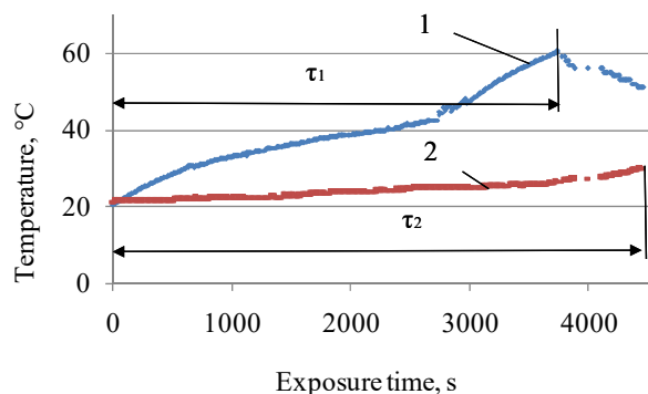
Fig. 7. Results of determining the temperature on the surface of a wood polymer material when heated to 60 °C: 1 – heating curve; 2 – temperature value on the inverted surface of the sample; points \tau_1 correspond to the value of the heating curve temperature rise time; \tau_2 – in accordance with the value of the temperature rise time on the inverted surface
