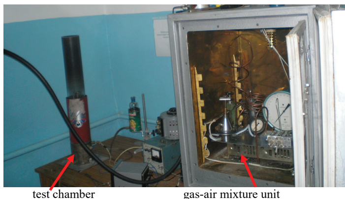
Fig. 2. Installation for determining the minimum fire extinguishing concentration
