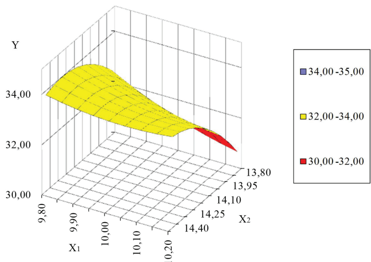
Fig. 7. Ternary surfaces of changes in the initial parameter depending on changes in the factors of variation in the amount of nitrogen and oxygen concentration
