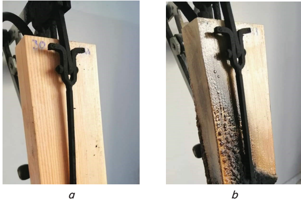
Fig. 2. Wood sample: a – before testing; b – after thermal action
