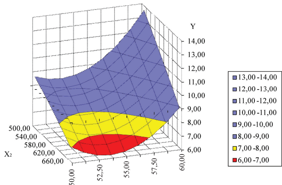
Fig. 4. Ternary surfaces of changes in the original parameter, depending on changes in the variance factors for the volume of protective coating
