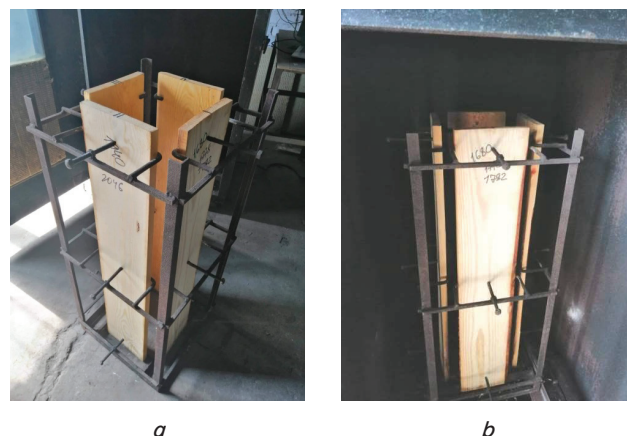
Fig. 5. Samples of wood during combustibility tests: a – before testing; b – after thermal action
