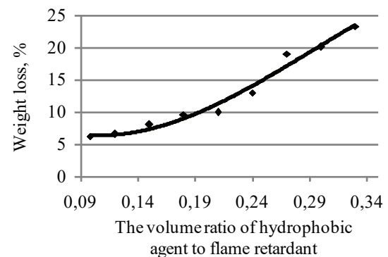
Fig. 3. Determining the mass loss (%) depending on the ratio of a hydrophobic agent to a flame retardant for pine wood samples
